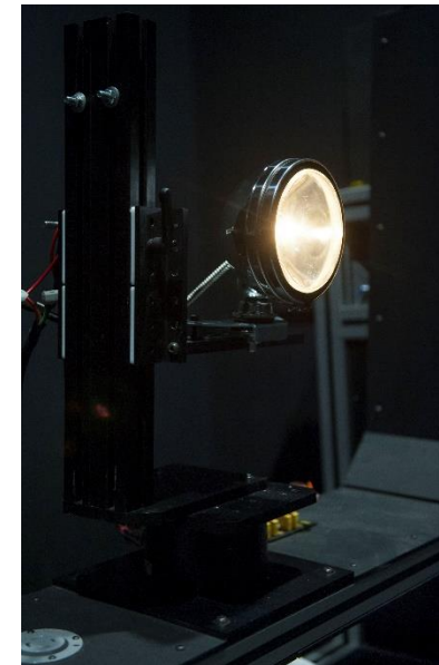
Horticulture Irradiance Gantry Type C Moving Mirror Goniometer Type A Goniometer
