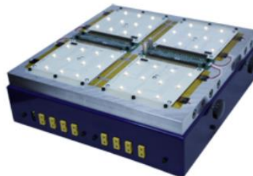
LM80 Thermal Platform
